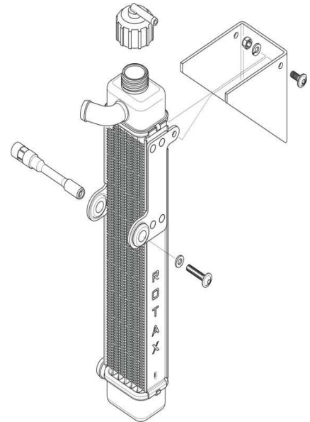
Version 2 Radiator
